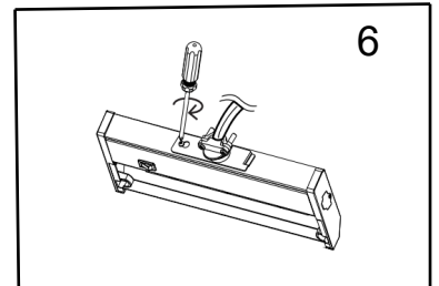
Feed wires back into the fixture, reattach the rear access door plate, tighten screw, and attach the fixture to the base of the cabinet with screws
