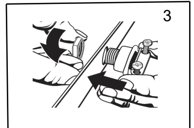
Insert the romex connector into the housing open hole on the rear access door plate. Secure it with the nut
