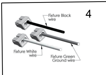
Pull 3 wires out of the fixture to allow connection to the branch circuit. Insert wires into the open hole in the push-in wire connector
