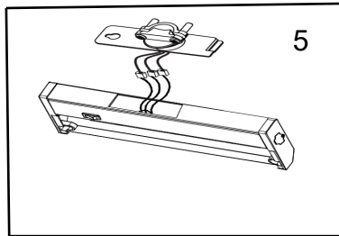
Connect the wires. Black to Black, white to white, Green to Green (Ground wire). Do not mix wires or change polarity
