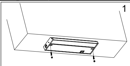
Fix the fixture to the unit using 2 fixture screws
